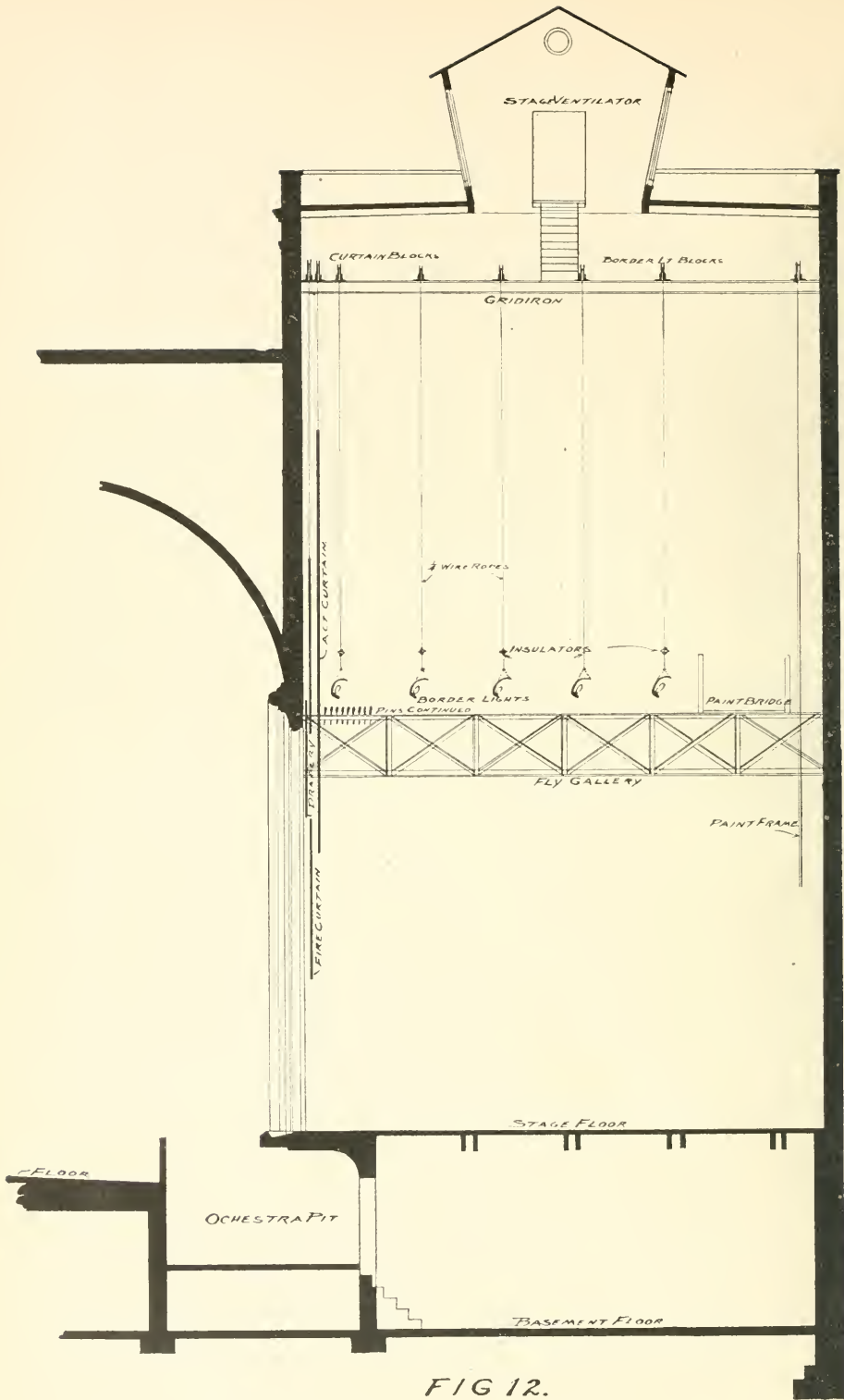
Showing a longitudinal section of the stage, with Fly Gallery, Gridiron, Paint Bridge, also indicating the relative position of the border lights. A type of stage ventilation is here suggested, with sides that fall to roof when released by breaking of the fusible link in case of fire.
